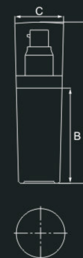
XLE-35I Capacity:35ml Height(A):131.2mm (B):87.5mm Diameter(C):40.0mm Discharge Rate:0.23ml
