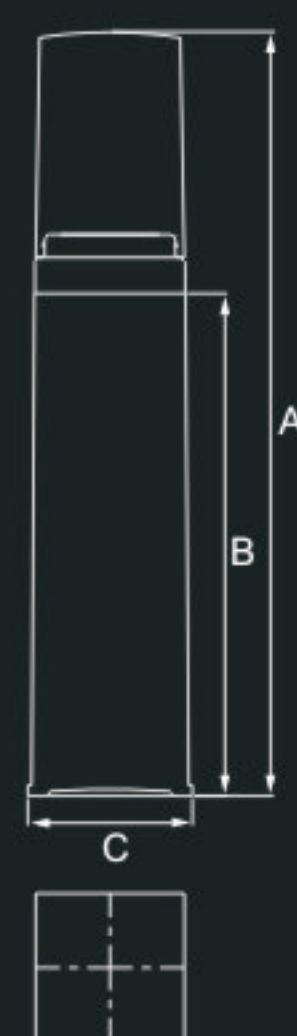
XLD-30A Capacity:30ml Height(A):160.0mm (B)112.7mm Diameter(C):31.2mm Discharge Rate:0.23ml
